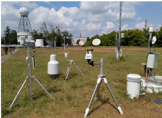
Instruments are tested at Marczell György Main Observatory (July 2025)
